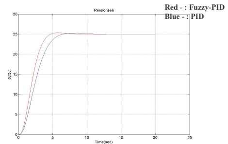
Fig. 8. Step Response of Surface Vessel Model
