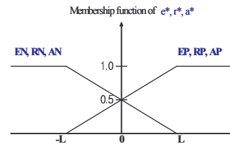
Fig. 6. Input Membership Function
