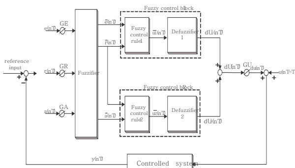
Fig. 5. Structure of Fuzzy-PID Controller
